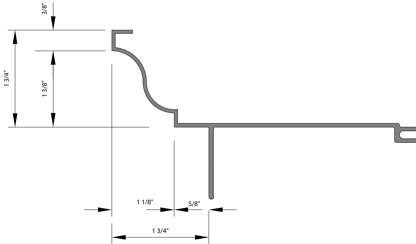
CROWN RECEPTOR
